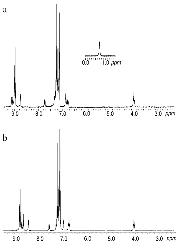
Figure 3. 1 H NMR spectra of dimeric phthalocyanines 9a (a) and 9b (b) in CDCl 3 .
