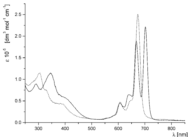
Figure 1. UV/Vis spectra ( \text{CH}_2\text{Cl}_2 ) of 7a (solid line) and 7b (dashed line).
