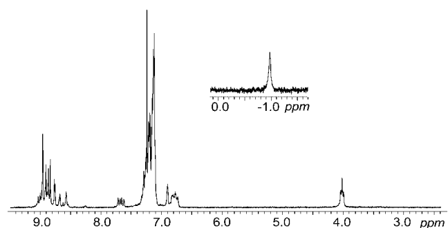
Figure 5. 1 H NMR spectrum of heteronuclear dimeric phthalocyanine 9c .
