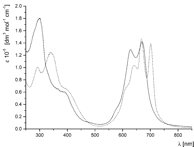
Figure 2. UV/Vis spectra ( \text{CH}_2\text{Cl}_2 ) of 9a (dashed line) and 9b (solid line).
