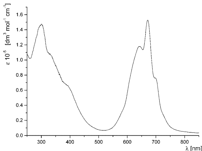
Figure 4. UV/Vis spectrum (CH 2 Cl 2 ) of dimer 9c .
